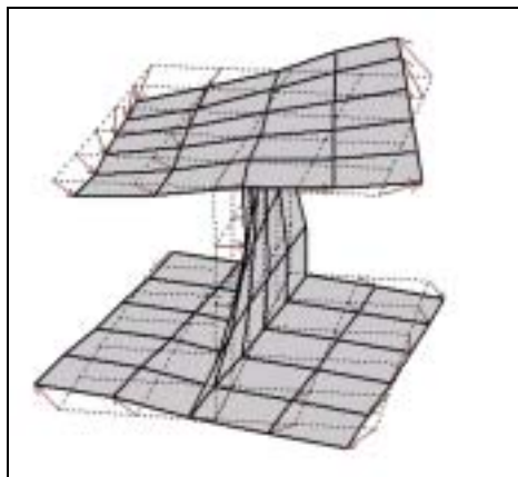
Fig. 10 Left: Mode shape for the 2nd mode with predominant, horizontal modal deflection
